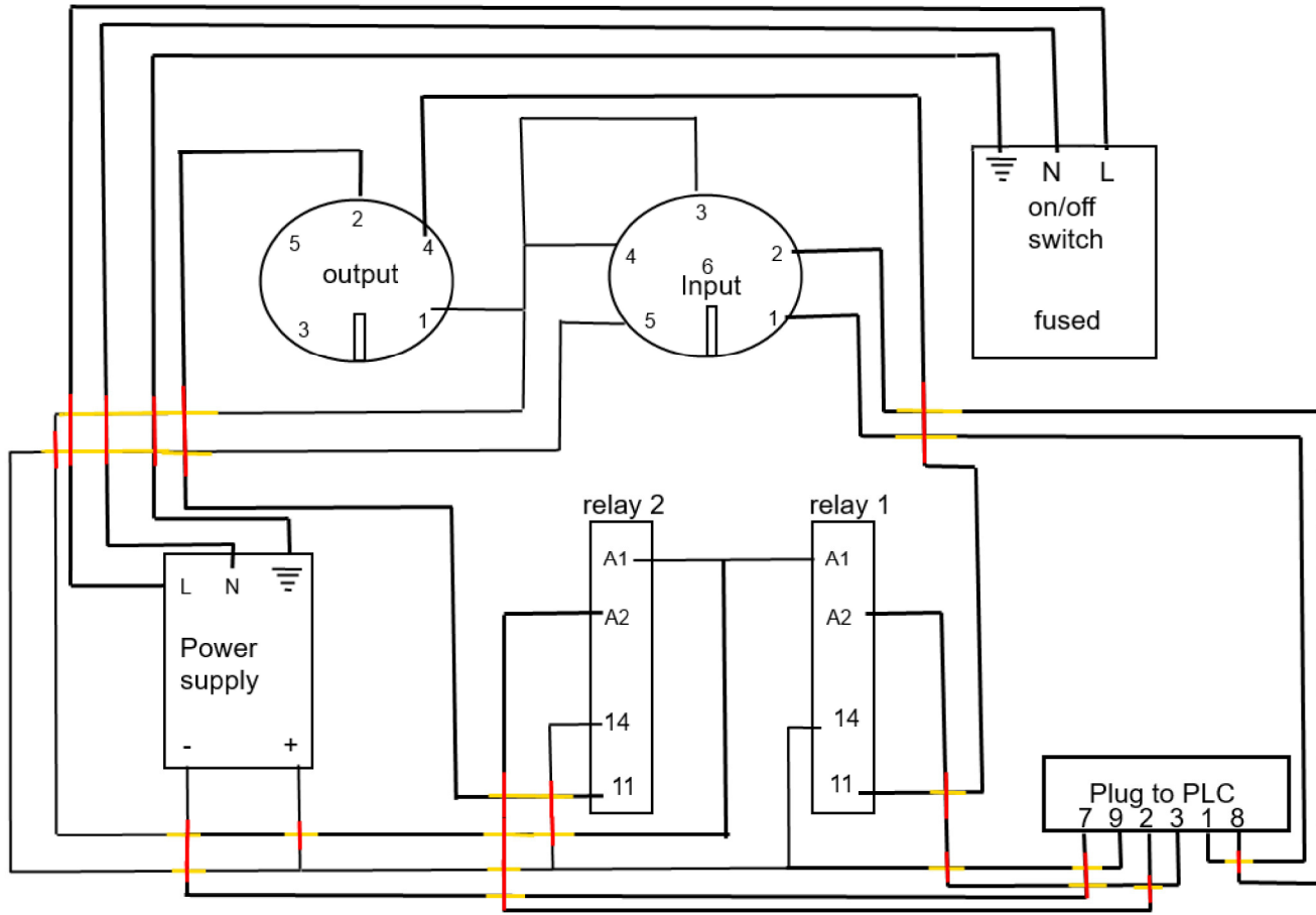
Shooter-IID ECU wiring diagram Rev1 October 2015
